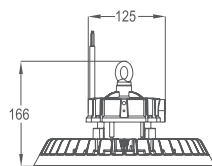
HELO PRO (S) 150W
