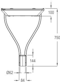
5005 GARDEN LIGHT (SOLAR SERIES)
