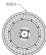
HELO PRO (L) 240W / 300W
