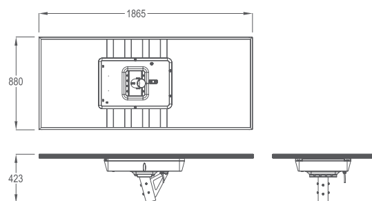
Titan712 Solar System 200W
