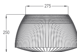
PC REFLECTOR + DIFFUSER
