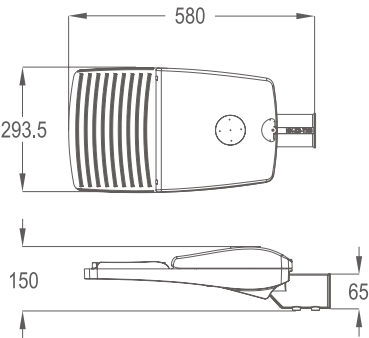
SIGMA-M PRO Side Entry
