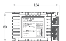
Light Control Unit
