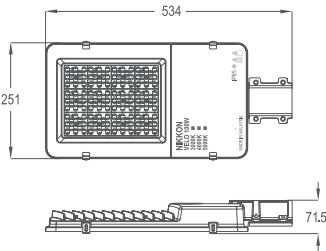
VELO 100W / 120W
