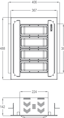
LEDXION K03108 160W
