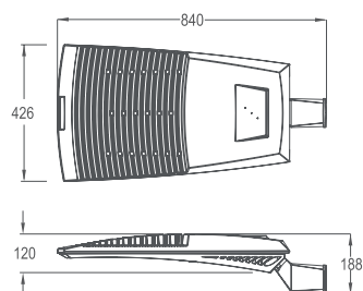
K09133 M2 - Side Entry
