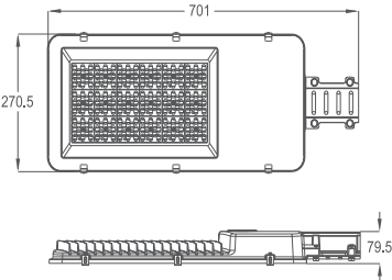
VELO 150W / 180W
