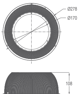
PC Reflector
