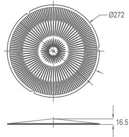
PC Visor
